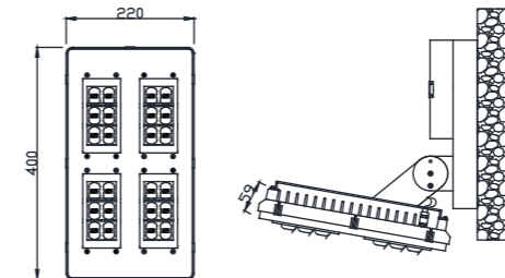
LED 60W
